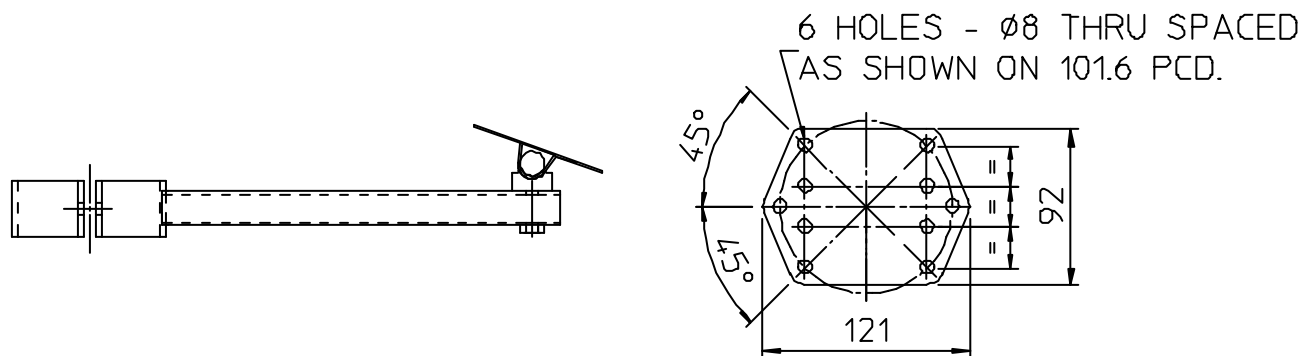
SWIVEL MOUNT DETAIL
